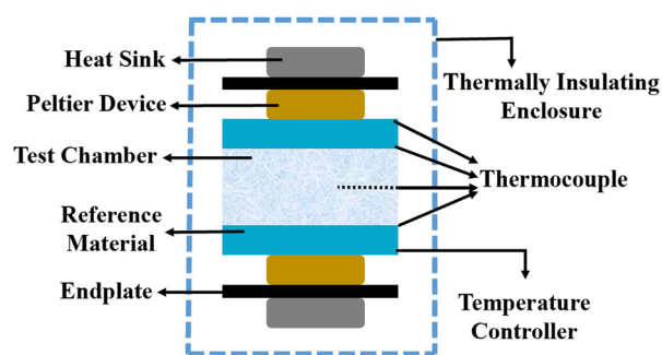
Fig. 12 Schematic diagram of the temperature oscillation technique. Adapted from ref. 96, with permission from Elsevier, Copyright 2021.
