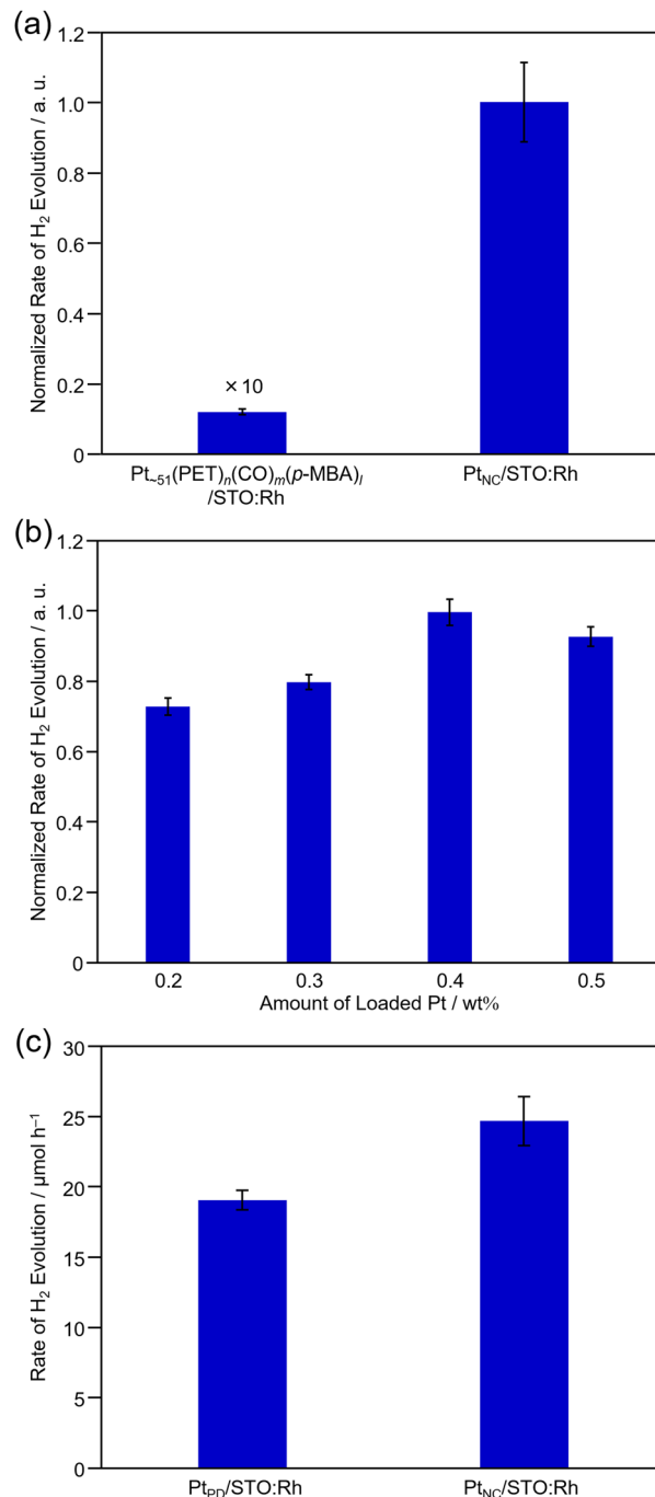
Fig. 5 H 2 -evolution activity of Pt cocatalyst-loaded STO:Rh photocatalysts. (a) Before ( \text{Pt}_{51}(\text{PET})_3(\text{CO})_3(p\text{-MBA})_3/\text{STO:Rh} ) and after ( \text{Pt}_{\text{NC}}/\text{STO:Rh} ) calcination of Pt NC-loaded STO:Rh and (b) dependence of loading weight of the Pt cocatalyst for \text{Pt}_{\text{NC}}/\text{STO:Rh} . (c) Comparison of H 2 -evolution activity between \text{Pt}_{\text{NC}}/\text{STO:Rh} and \text{Pt}_{\text{PD}}/\text{STO:Rh} . In (a) and (c), the loading weight of Pt on them was 0.4 wt%. In order to eliminate the effect of the difference in the activity of each photocatalyst, STO:Rh synthesized in the same batch was used in each experiment (a)–(c).
