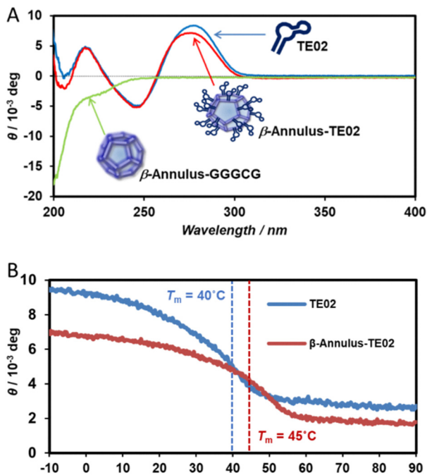
Fig. 3 (A) CD spectra of 20 \mu\text{M} \beta -Annulus-TEO2 (red), \beta -Annulus-GGGCG (green), and TEO2 (blue) in 10 mM phosphate buffer at 25 ^{\circ}\text{C} . (B) Temperature dependence in ellipticity at 270 nm of TEO2 (blue) and \beta -Annulus-TEO2 (red).
