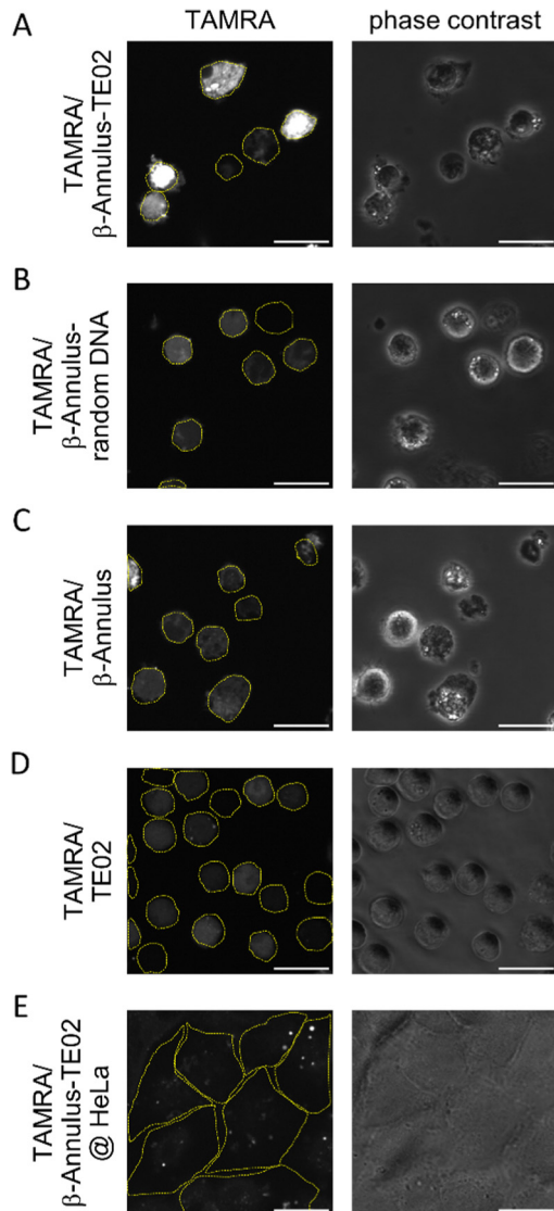
Fig. 4 (A)–(D) CLSM images of Daudi cells treated using (A) TEO2-decorated capsid (TAMRA/ \beta -Annulus-TEO2), (B) random DNA-decorated capsid (TAMRA/ \beta -Annulus-random DNA), (C) unmodified capsid (TAMRA/ \beta -Annulus) and (D) TAMRA/TEO2. (E) CLSM image of HeLa cells treated using TEO2-decorated capsid (TAMRA/ \beta -Annulus-TEO2). TAMRA fluorescence was shown as white. Yellow dashed lines; cellular boundaries. Scale bars; 20 \mu\text{m} .
