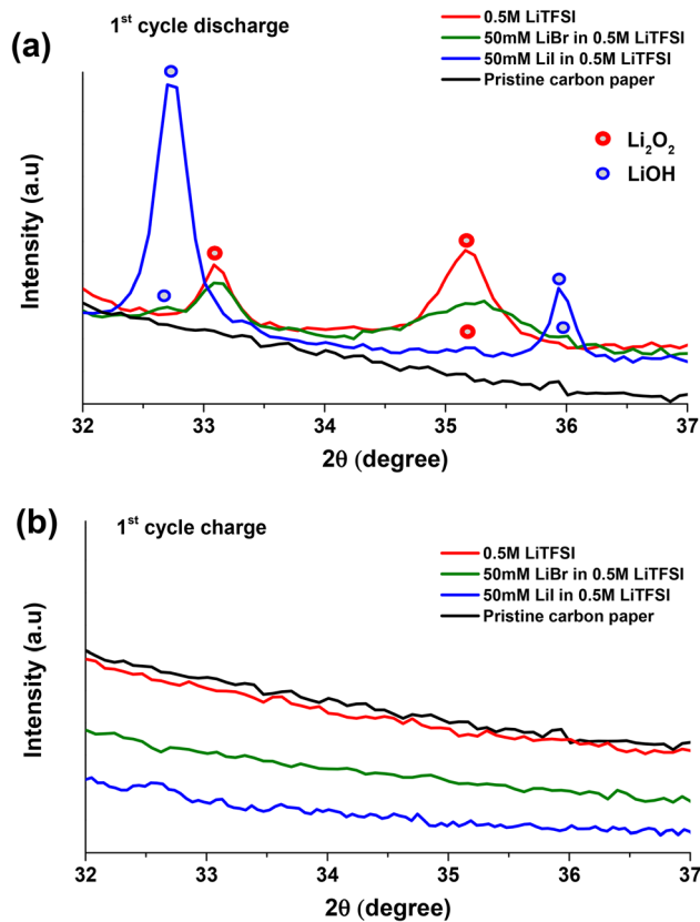
Fig. 3 X-ray diffraction spectra of Li–O 2 cells with 0.5 M LiTFSI, 50 mM LiI in 0.5 M LiTFSI and 50 mM LiBr in 0.5 M LiTFSI in diglyme solutions after (a) first cycle discharge and (b) the subsequent charge under O 2 .
