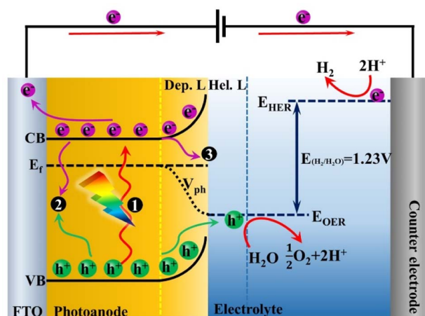
Fig. 1 The principles of PEC water splitting for single photoanode configurations under light irradiation. Mark 1 represents the process of charge separation under light irradiation. Marks 2 and 3 represent the bulk and surface recombination, respectively. Dep. L: depletion layer, Hel. L: Helmholtz layer, CB: conduction band, E_f : Fermi energy level, VB: valence band, and V_{ph} : photo-potential.
