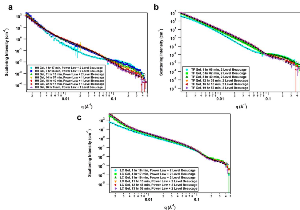
Fig. 6 (a) Time-resolved SANS data of HH-Gel , fitted with a summed unsmoothed power law + 2 level Unified model for the first three time points and then power law + 1 level for the remaining four time points. (b) Time-resolved SANS data of TF-Gel , fitted with a summed unsmoothed 2 Level model. (c) Time-resolved SANS data of LC-Gel , fitted with a summed unsmoothed power law + 2 level model.
