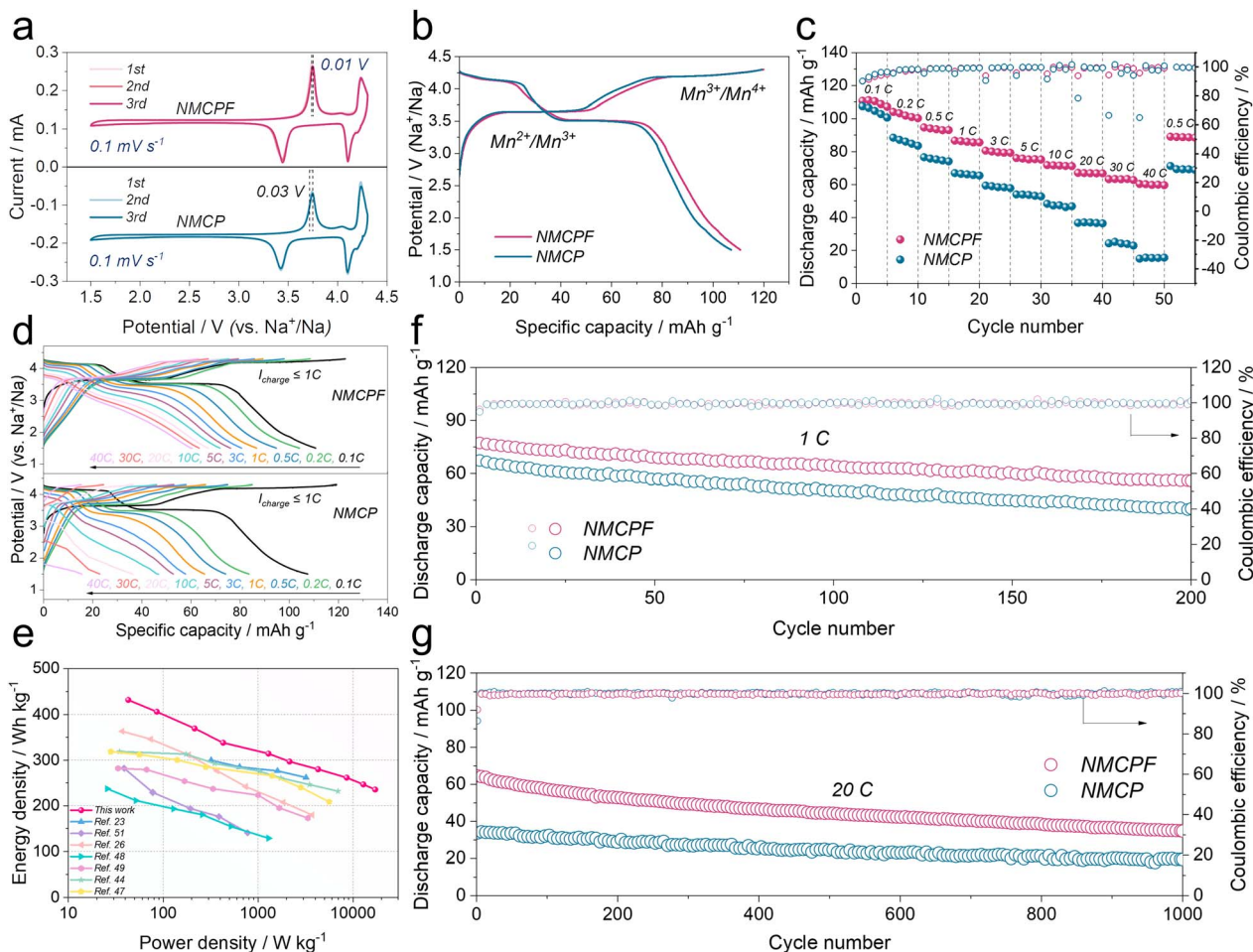
Fig. 4 Electrochemical capabilities within 1.5–4.3 V. (a) CV curves at 0.1 \text{ mV s}^{-1} . (b) Initial charge/discharge curves at 0.1\text{C} ( 1\text{C} = 110 \text{ mA h g}^{-1} ). (c) Rate properties. (d) Charge/discharge profiles at various rates. (e) Ragone plot. Cycling capabilities at (f) 1\text{C} and (g) 20\text{C} .
