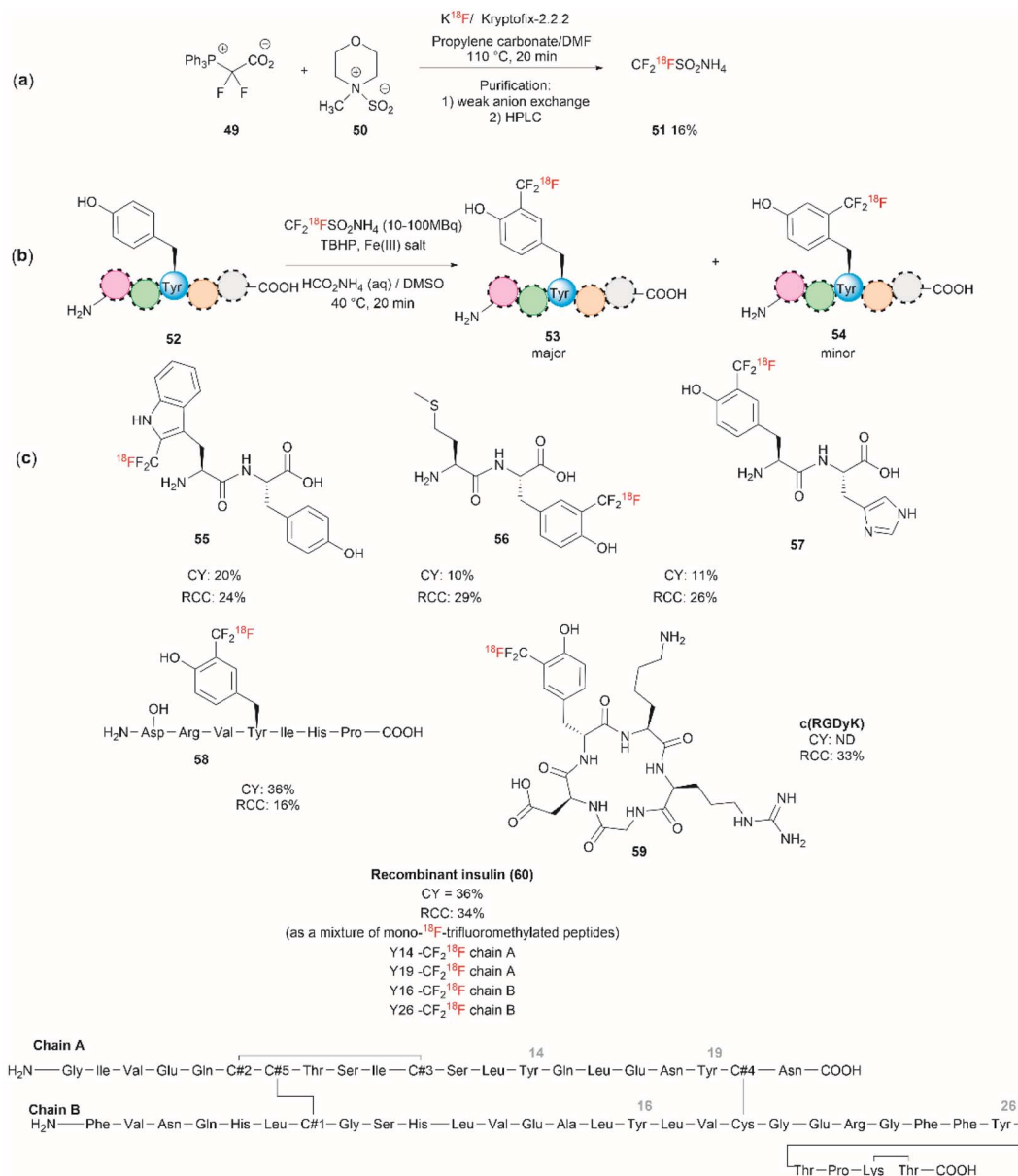
Fig. 13 (a) Chemical synthesis of ammonium ^{18}\text{F} -trifluoromethanesulfinate. (b) General conditions for the ^{18}\text{F} -trifluoromethylation of Tyr containing peptides. (c) ^{18}\text{F} -trifluoromethylated peptides.
