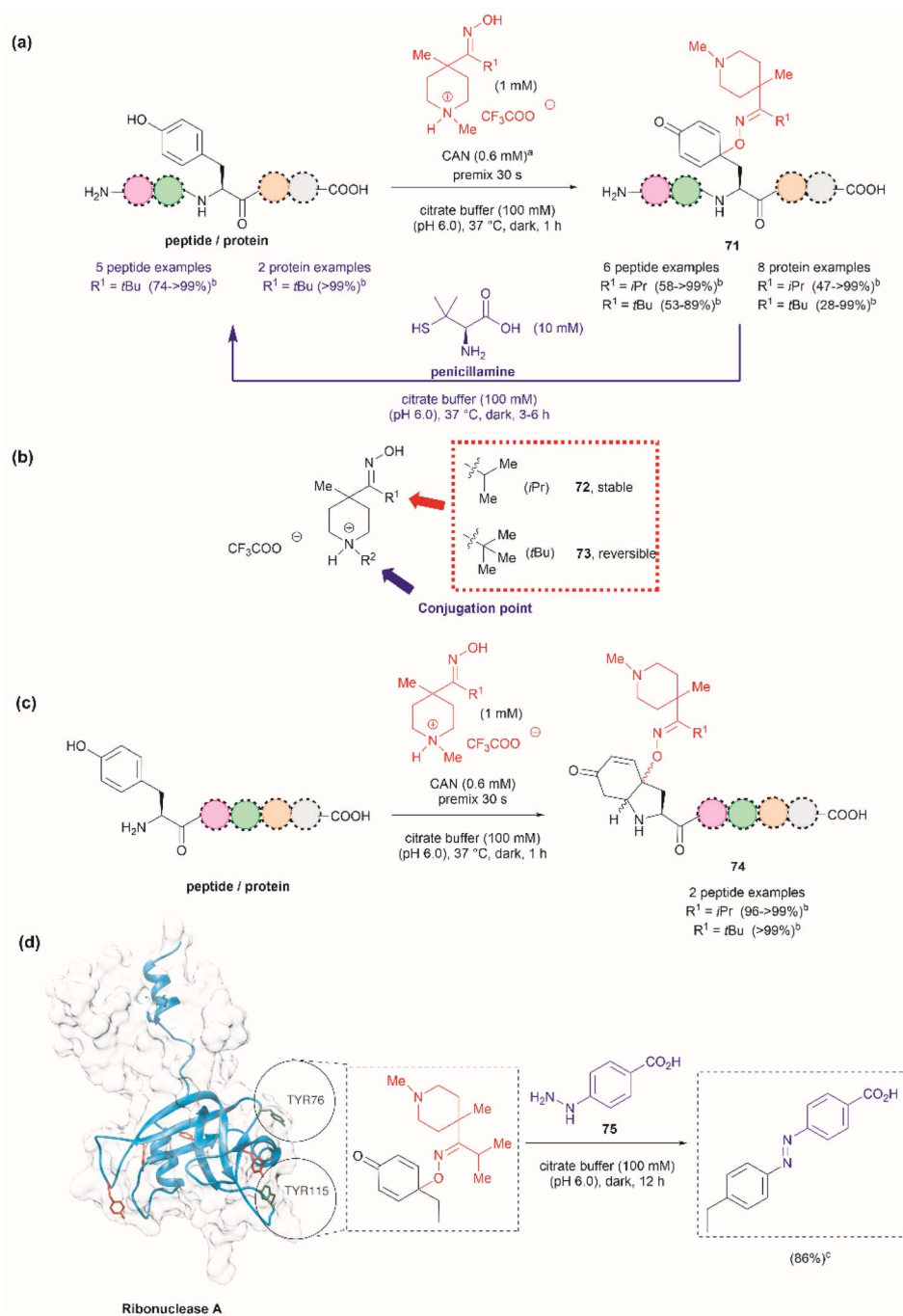
Fig. 17 (a) Reaction conditions for the formation of cyclohexadienone adducts in Tyr-containing peptides/proteins and conditions for the reversible reaction to Tyr (blue arrow). a Thiourea (5 mM) was added to minimize oxidation of proteins and peptides containing Met. b Conversion determined by the HPLC peak area. (b) Structural modification points of the water soluble 4-methylpiperidinium oximes. (c) Post cyclization of the cyclohexadienone adduct in peptides containing Tyr at the N-terminus. (d) Introduction of benzodiazo substituents in ribonuclease A (PDB: 1A2W) cyclohexadienone adducts. For clarity the figure only shows one of the chains of the dimeric form of the protein. Tyr residues that are not modified by the iminoxyl radicals are colored in red and Tyr residues forming adducts with the radicals are labeled and shown in green. c Calculated yield determined by LC-MS analysis.
