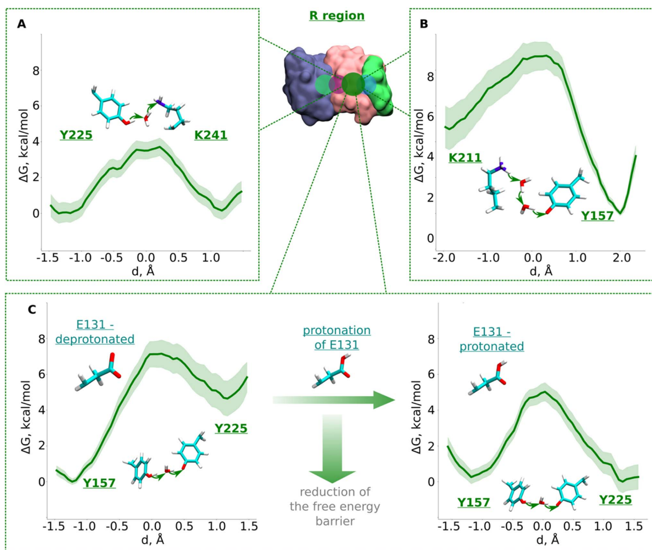
Fig. 3 Free energy profiles of proton transfer from conserved Lys/Glu pair to central lysine (R region). (A) Tyr225 (neutral) → H 2 O → Lys241 (neutral) pathway. (B) Lys211 (protonated) → H 2 O → H 2 O → Tyr157 (deprotonated) pathway. (C) Proton transfer from Tyr157 (neutral) through H 2 O to Tyr225 (deprotonated). The left panel shows energetics when Glu131 of conserved Lys/Glu pair is deprotonated, and when protonated (right panel). The bold green lines are PMF profiles with light green shaded area highlighting the bootstrapping error range (see also methods). Occupational histograms for the reaction coordinates are given in ESI, Fig. S17B–E. \dagger Inset shows ND4, ND2, and ND4L subunits in blue, pink, and green surface representation, respectively. The QM region where the proton transfer is studied is marked with the dark green circle.
