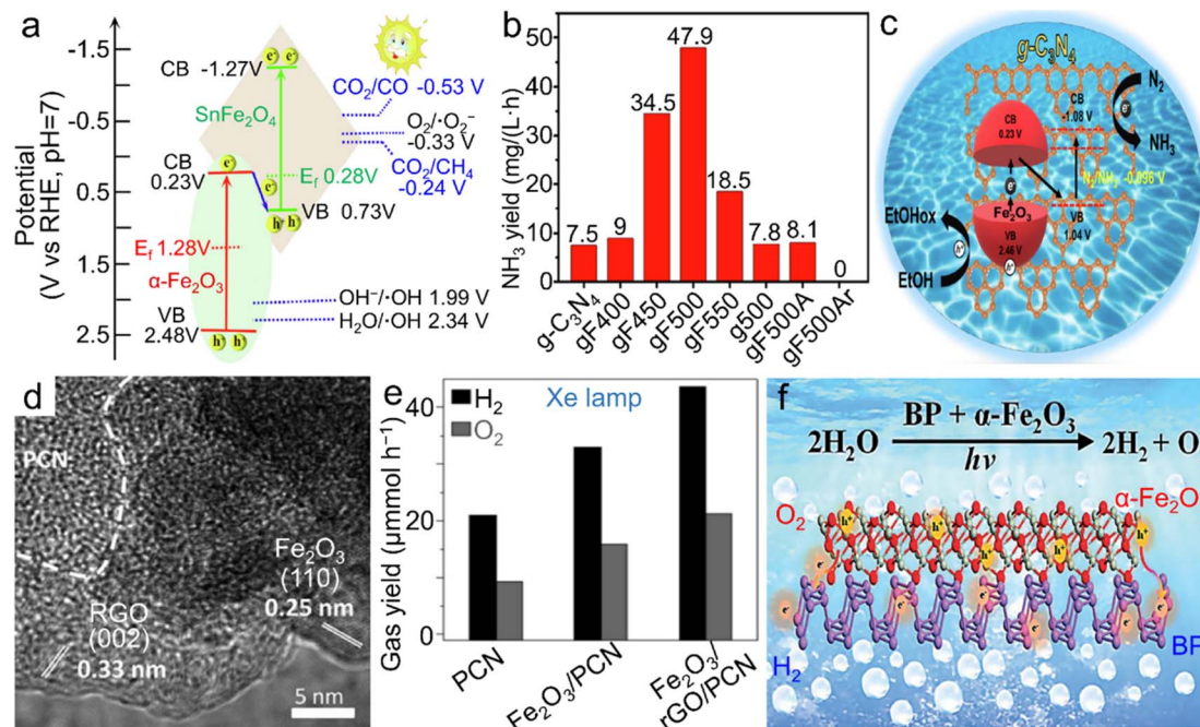
Fig. 7 \alpha\text{-Fe}_2\text{O}_3 materials for photocatalytic reactions. (a) Band structure of the Z-scheme \alpha\text{-Fe}_2\text{O}_3/\text{SnFe}_2\text{O}_4 heterostructure for photocatalytic \text{CO}_2 RR into CO and \text{CH}_4 . Adapted with permission from ref. 145. Copyright 2020, Elsevier Inc. (b) Photochemical \text{NH}_3 yield rate of both pristine g\text{-C}_3\text{N}_4 and \alpha\text{-Fe}_2\text{O}_3/g\text{-C}_3\text{N}_4 calcined at different temperatures and/or atmospheres and (c) the scheme for electronic band structure of \alpha\text{-Fe}_2\text{O}_3/g\text{-C}_3\text{N}_4 towards photocatalytic \text{N}_2 fixation. (b and c) Adapted with permission from ref. 151. Copyright 2019, John Wiley & Sons, Inc. (d) TEM image and (e) photocatalytic overall water splitting rate of the \alpha\text{-Fe}_2\text{O}_3/\text{rGO}/\text{PCN} composite. (d and e) Adapted with permission from ref. 156. Copyright 2019, John Wiley & Sons, Inc. (f) Scheme of the \text{BP}/\alpha\text{-Fe}_2\text{O}_3 photocatalyst for photochemical overall water splitting. Adapted with permission from ref. 157. Copyright 2021, Royal Society of Chemistry.
