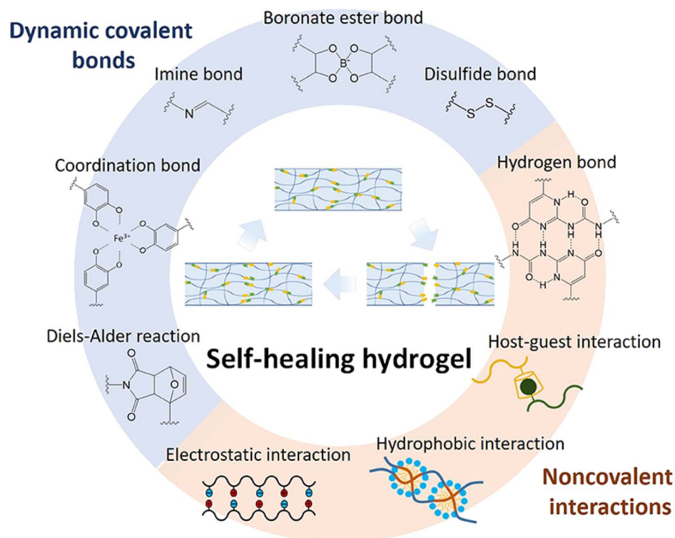
Fig. 4 Summary of self-healing mechanisms employed in hydrogels. 126 This figure has been adapted/reproduced from ref. 126 with permission from Frontiers in Chemistry , copyright 2023.
