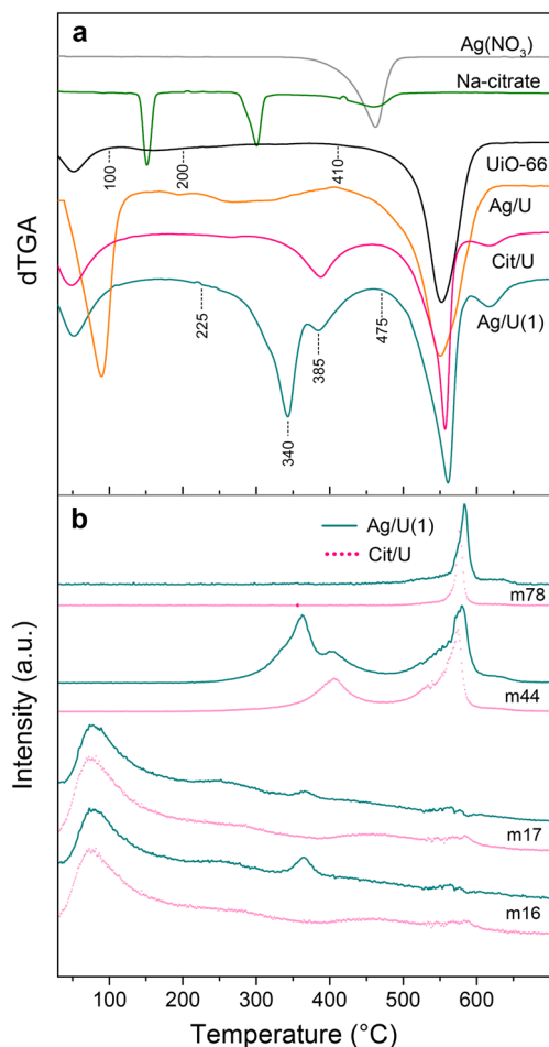
Fig. 2 a) TGA derivative profiles (dTGA); b) TGA-MS for Ag/U(1) (solid line) and Cit/U (dotted line). Note: m16 ( \text{O}_2 , \text{H}_2\text{O} ); m17 (OH, \text{H}_2\text{O} ); m44 ( \text{CO}_2 ); m78 ( \text{C}_6\text{H}_6 ).
