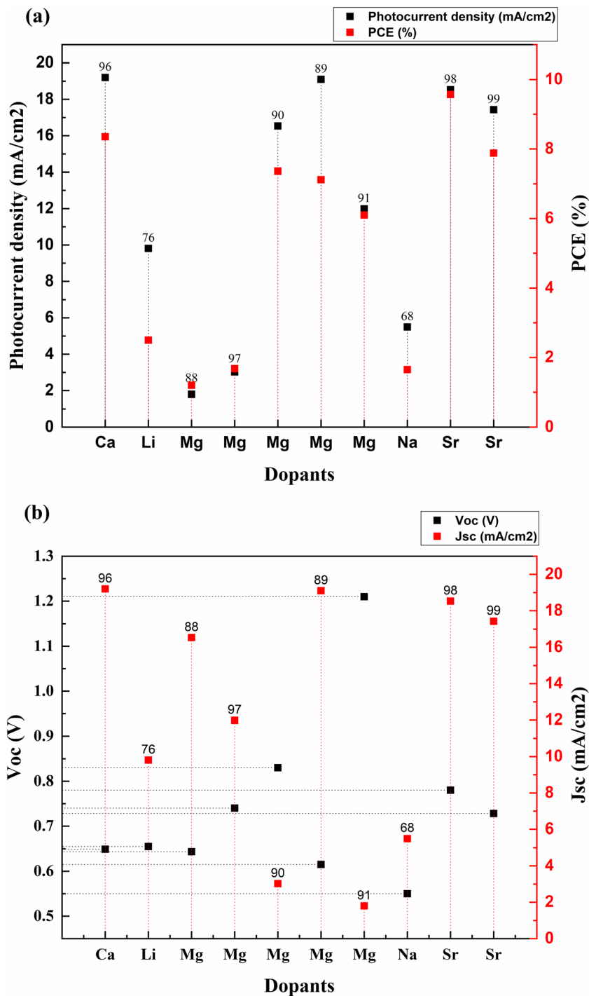
Fig. 7 (a) Performance of alkali & alkaline earth metal doped TiO 2 based DSSCs. (b) V oc and J sc values of alkali & alkaline earth metal doped TiO 2 based DSSCs. Data points are labelled with references.
