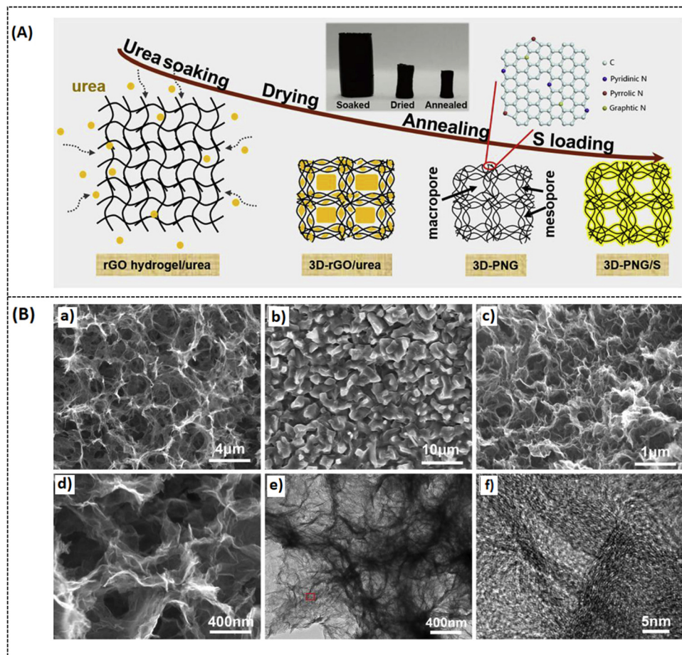
Fig. 6 (A) Schematic illustration of the preparation process of 3D-PNG/S composites, (B) (a and b) SEM images of 3D-rGO, 3D-rGO@ures, (c and d) low-magnification SEM of 3D-PNG (e and f) TEM image of 3D-PNG, HRTEM image of the marked area in (e). Reprinted with permission, 56 Copyright (2019) from Elsevier.
