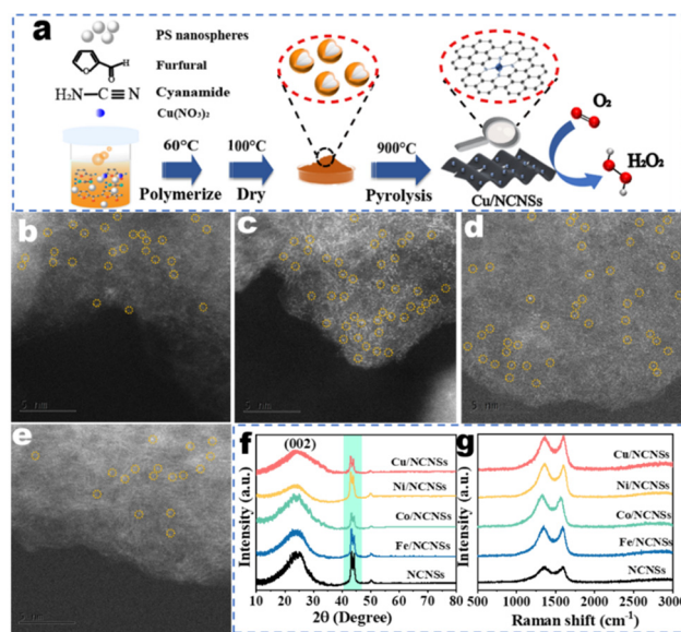
Fig. 1 The synthetic process of M/NCNSs (a), high-resolution HAADF-STEM images of Fe/NCNSs (b), Co/NCNSs (c), Ni/NCNSs (d), and Cu/NCNSs (e), XRD patterns (f) and Raman spectra (g) of the as-synthesized samples.
