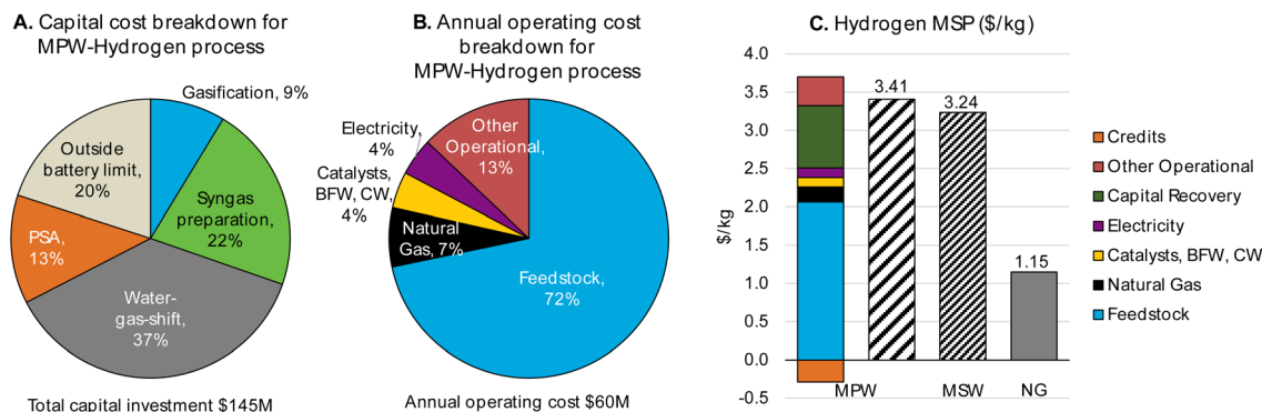
Fig. 5 CAPEX, OPEX, and MSP breakdown for MPW-hydrogen process (MPW: 240 MT per D feedstock, 70 MT per D hydrogen). (A) Detailed breakdown of CAPEX by process section is given in Table S12. † (B) A detailed breakdown of OPEX for variable and fixed costs is given in Table S13. † (C) A comparison of MSP for MPW-Hydrogen, MSW-hydrogen, and natural gas (NG)-based processes. The breakdown and net MSP for the MPW-hydrogen process are shown in separate bars. In the MSW-hydrogen case, the feedstock cost is zero. A detailed MSP breakdown by process section is given in Table S14. †
