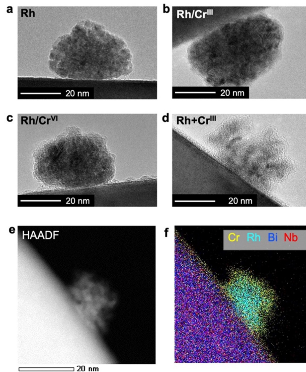
Fig. 2 HR-TEM images of cocatalysts loaded on (a) Rh, (b) Rh/Cr III , (c) Rh/Cr VI , and (d) Rh + Cr III samples. (e) HAADF-STEM and (f) EDX elemental mapping images of the Rh + Cr III sample.
