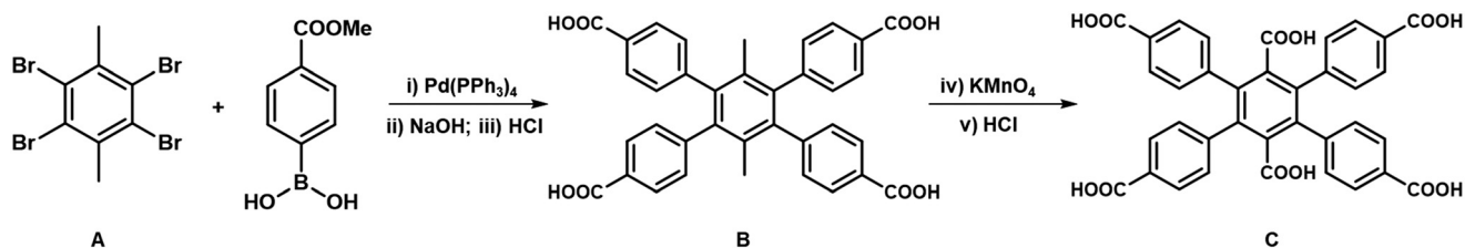
Scheme 1 Synthesis of 1,2,4,5-tetrakis(4-carboxyphenyl)-3,6-dicarboxyl-benzene (H 4 tcpb-(COOH) 2 ).
