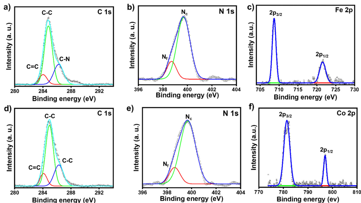
Fig. 2 (a–c) C 1s, N 1s, and Fe 2p XPS spectra of ITO/tpy- [\text{Fe}(\text{bis-tpy})]_5 and (d–f) C 1s, N 1s, and Co 2p XPS spectra of ITO/tpy- [\text{Co}(\text{bis-tpy})]_5 . The solid lines represent fitted data, while the open circles indicate experimental data. \text{N}_f and \text{N}_c stand for free nitrogen and coordinated nitrogen that binds metal ions ( \text{Fe}^{2+} or \text{Co}^{2+} ).
