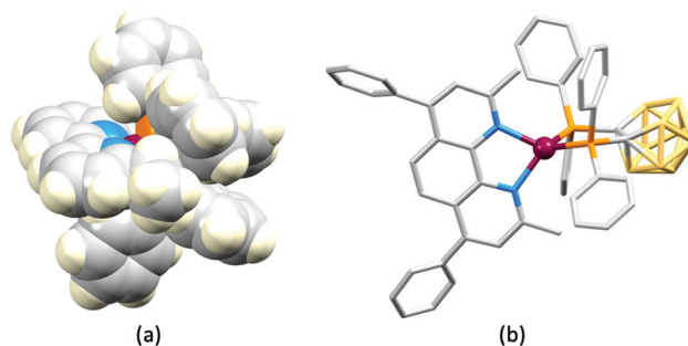
Fig. 20 (a) Structure of the cation in [Cu(BIPHEP)(6-Etbpy)][PF 6 ] in space-filling representation (CSD refcode WOXHEZ). (b) Structure of [Cu(dppnc)(2,9-Me 2 -4,7-Ph 2 phen)][PF 6 ] (CSD refcode MUJXOG) with H atoms omitted.
