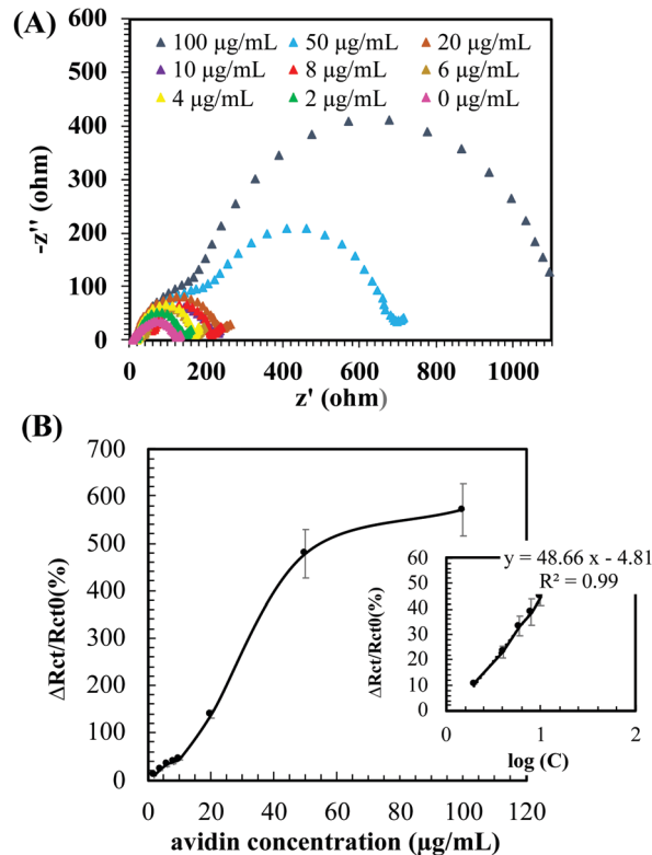
Fig. 7 (A) Impedance Nyquist plots of the EIS from ITO modified with PG/b-pSBAE ( 8/30 \text{ mg mL}^{-1} ) after immersion in avidin solution at various concentrations ( 0 – 100 \text{ }\mu\text{g mL}^{-1} ). Measurements were performed in PBS containing 10 \text{ mM } [\text{Fe}(\text{CN})_6]^{3-/4-} and 0.1 \text{ M KCl} . (B) Changes in the charge transfer resistance [ \Delta R_{ct}/R_{ct0} (%)] of the PG/b-pSBAE modified ITO after immersion in avidin solution at various concentrations. Inset: the corresponding regression curve of the PG/b-pSBAE modified ITO. C: Avidin concentration. Value = mean \pm standard deviation, n = 3 .
