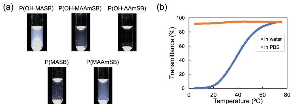
Fig. 2 (a) Photo images of sulfobetaine polymer solutions in water. (b) Transmittance of P(OH-MASB) solutions as a function of temperature. The cooling rate of the solutions was 1.0 \text{ } ^\circ\text{C min}^{-1} . [Polymer] = 10 \text{ g L}^{-1} .
