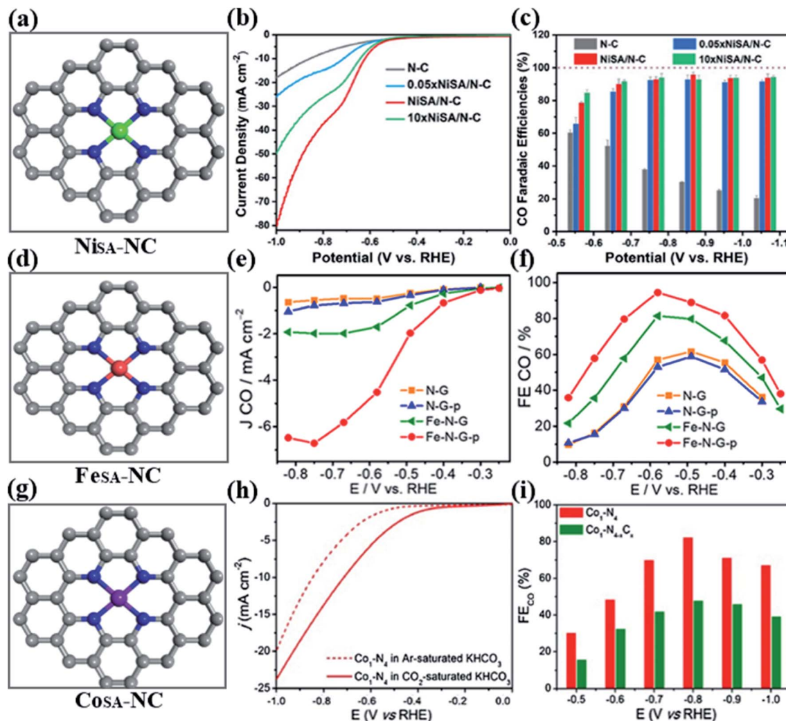
Fig. 2 (a) Structural model of \text{Ni}_{\text{SA}}\text{-NC} SACs. (b) Linear sweep voltammetry (LSV) curves at a scan rate of 10 \text{ mV s}^{-1} . (c) \text{FE}_{\text{CO}} for \text{N-C} , 0.05\text{xNi}_{\text{SA}}/\text{N-C} , \text{Ni}_{\text{SA}}/\text{N-C} , and 10\text{xNi}_{\text{SA}}/\text{N-C} catalysts tested in \text{CO}_2 -saturated 0.1 \text{ M KHCO}_3 electrolytes. Reproduced with permission from ref. 53. Copyright 2020, Elsevier. (d) Structural model of \text{Fe}_{\text{SA}}\text{-NC} SACs. (e) \text{CO} partial current density. (f) \text{FE}_{\text{CO}} for \text{N-G} , \text{N-G-p} , \text{Fe-N-G} , and \text{Fe-N-G-p} . Reproduced with permission from ref. 55. Copyright 2020, American Chemical Society. (g) Structural model of \text{Co}_{\text{SA}}\text{-NC} SACs. (h) LSV curves of \text{Co}_1\text{-N}_4 were recorded in \text{CO}_2 -saturated and \text{Ar} -saturated 0.1 \text{ M KHCO}_3 ( \text{pH} = 6.8 ) electrolytes. (i) \text{FE}_{\text{CO}} at selected potentials on \text{Co}_1\text{-N}_4 and \text{Co}_1\text{-N}_{4-x}\text{C}_x . Reproduced with permission from ref. 56. Copyright 2019, Elsevier.
