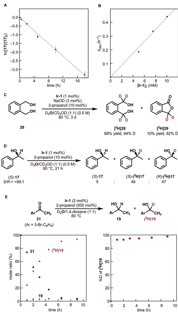
Fig. 3 Mechanistic studies. (A) Pseudo-first-order plot of H/D exchange of 1-phenylethanol ( 17 ) under the conditions III shown in Fig. 2. Average of three separate runs with standard deviations. (B) The observed rate constants ( k_{\text{obs}} , \text{h}^{-1} ) for deuteration of 17 plotted against [\text{Ir-1}]_0 (mM, 1–2 mol% Ir). (C) Lactone formation from diol 28 . (D) Racemization in the deuteration of ( S )-1-phenylethanol ( 17 ). (E) Reaction time course of reductive carbonyl deuteration with 2-propanol and \text{D}_2\text{O} : (left) molar ratio of 19 and 31 ; (right) % D at the \alpha carbon of [\text{2H}]\text{19} .
