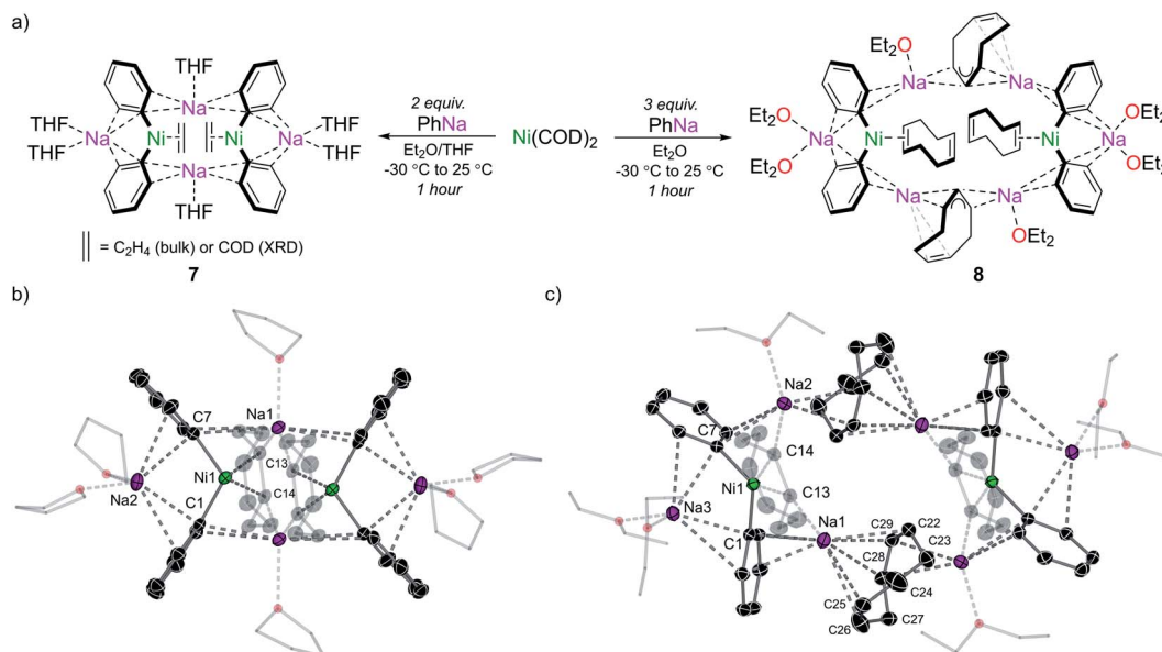
Fig. 7 (a) Reactions of Ni(COD) 2 with PhNa for the synthesis of [Na 2 (THF) 3 Ph 2 Ni(olefin)] 2 (7) and identification of [Na 2 (Et 2 O) 3 Ph 2 (-NaC 8 H 11 )Ni(COD)] 2 (8); (b) solid-state structure of 7. Thermal ellipsoids shown at 30% probability. Hydrogen atoms omitted and THF rings drawn as wireframes for clarity; (c) solid-state structure of 8. Thermal ellipsoids shown at 30% probability. Hydrogen atoms omitted and Et groups drawn as wireframes for clarity.
