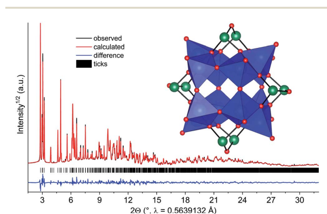
Fig. 7 Difference plot of the final Rietveld refinement for [\text{Ni}(\text{en})_3]_2[\text{As}_8\text{V}_6\text{O}_{26}(\text{H}_2\text{O})] \cdot 4\text{H}_2\text{O} with a final R_{\text{wp}} of 4.7% and R_{\text{Bragg}} = 3.7\% . The inset shows the polyhedral representation of the cluster anion in the structure of 2 . Note: the \text{H}_2\text{O} molecule in the cavity of the cluster is not displayed. Blue: \text{VO}_5 polyhedra; green: As; red: O.
