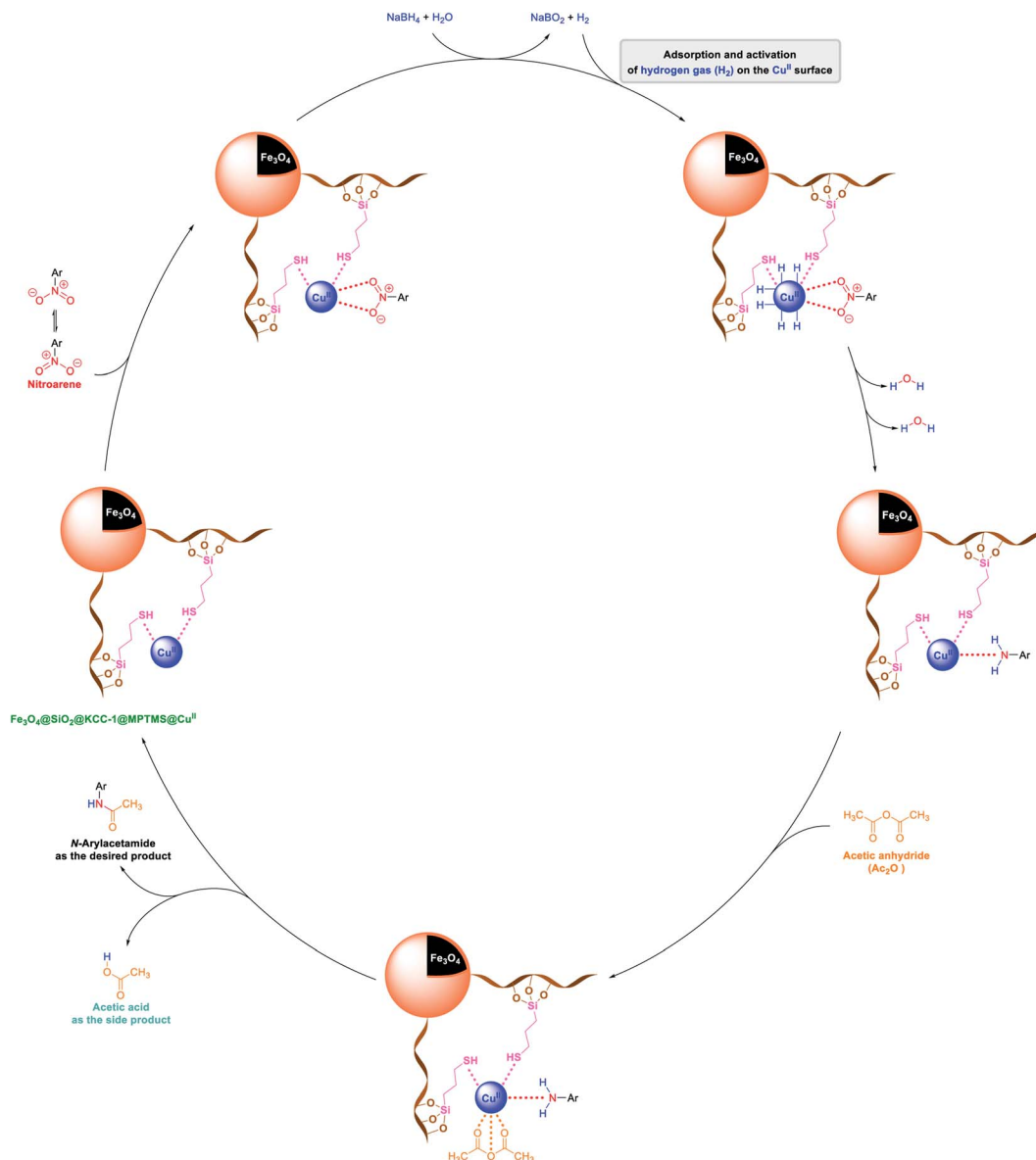
Scheme 2 Plausible mechanism of the one-pot reductive acetylation of nitroarenes catalyzed by the Fe 3 O 4 @SiO 2 @KCC-1@MPTMS@Cu II nanocomposite in water.
