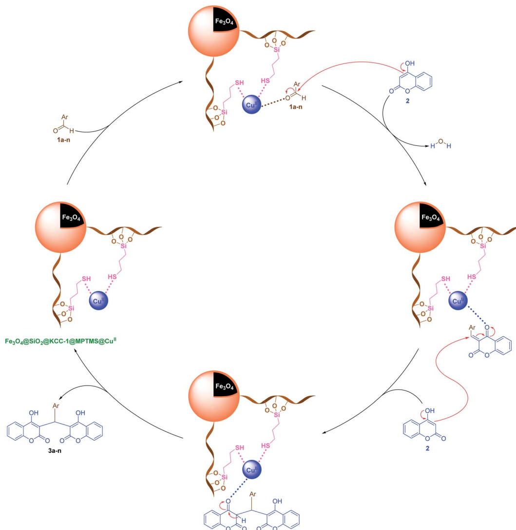
Scheme 5 Plausible mechanism for the solvent-free one-pot pseudo -three-component synthesis of bis-coumarins ( 3a-n ) catalyzed by the \text{Fe}_3\text{O}_4 @ \text{SiO}_2 @KCC-1@MPTMS@ \text{Cu}^{\text{II}} nanocomposite.
