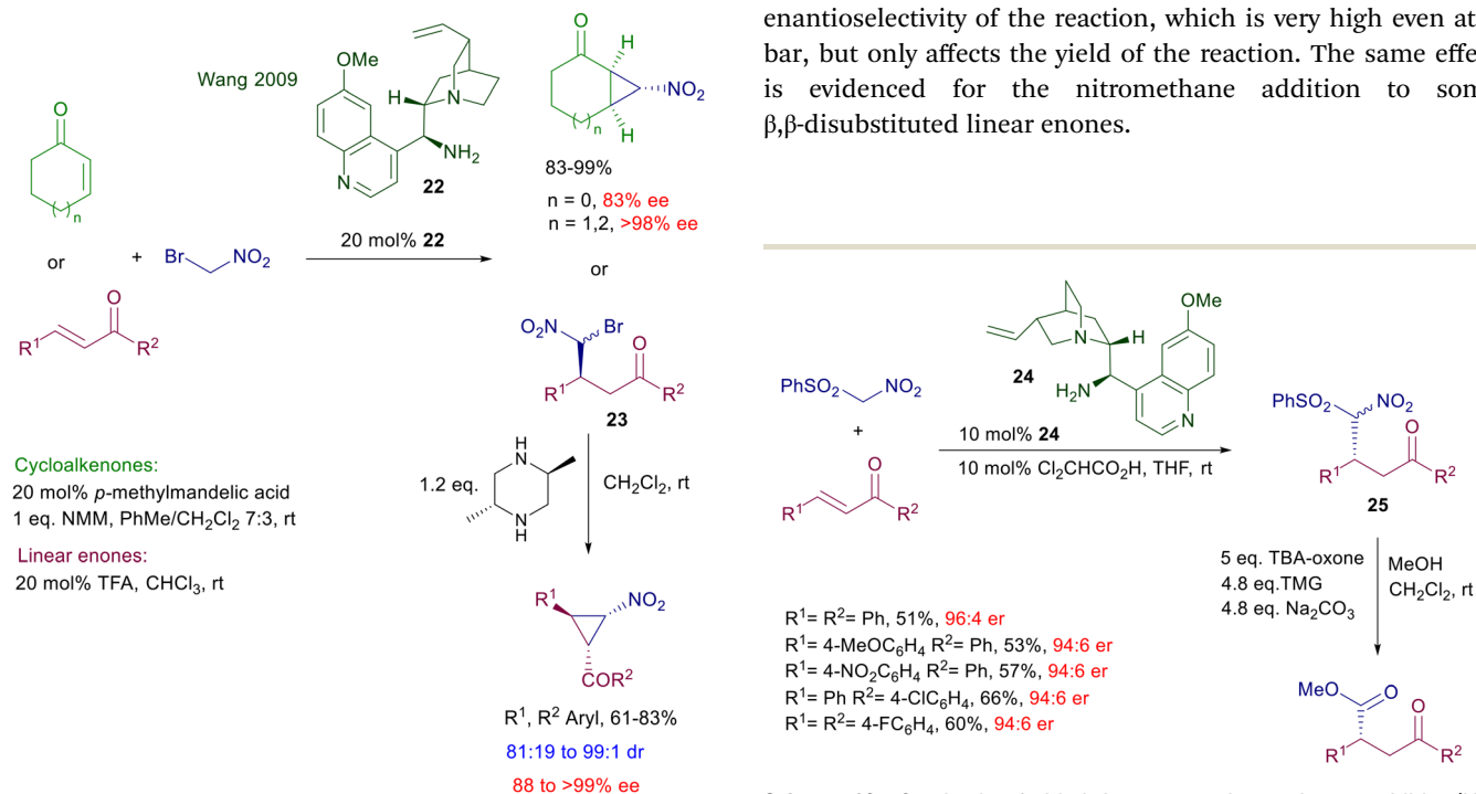
Scheme 19 Synthesis of chiral 4-oxoesters by conjugate addition/Nef reaction.
