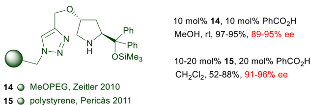
Scheme 9 Structural modifications of chiral prolinol catalysts.
