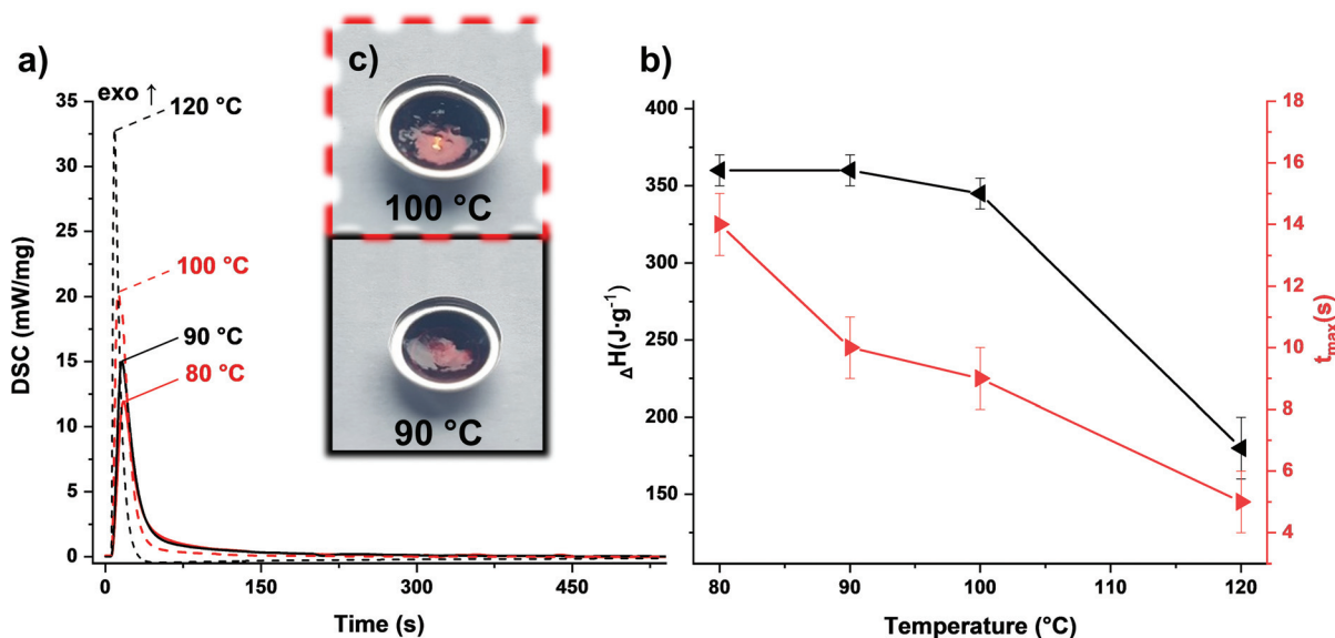
Fig. 5 (a) Photo-DSC of the TOMDA-formulation at 80–120 °C, 2 × 900 s, 320–500 nm, 60 \text{mW}\cdot\text{cm}^{-2} . (b) Temperature dependence of photo-DSC results for the TOMDA-formulation: enthalpy change ( \Delta H black) and time until maximal heat is released ( t_{\max} red). (c) Cured Samples at 90 & 100 °C.
