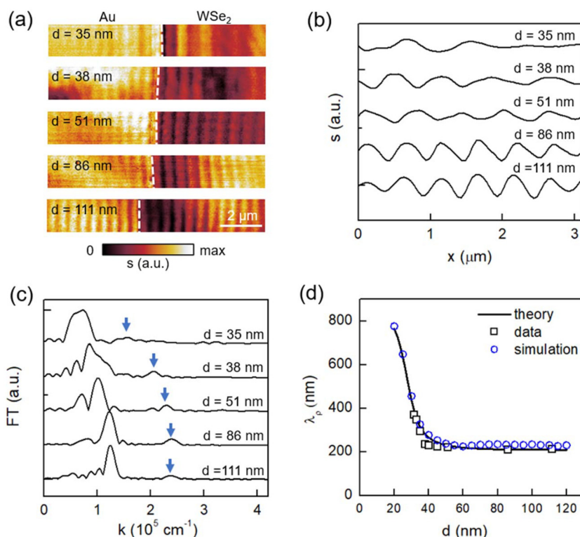
Fig. 3 (a) The near-field amplitude images of WSe 2 /Au heterostructure waveguides with various WSe 2 thicknesses ( d ). The excitation E was set to be E = 1.38 eV. (b) The fringe profiles (background subtracted) extracted from near-field images in panel (a). (c) Fourier-transform of the fringe profiles in panel (b). The arrows mark the peak associated with EPP interference involving beam paths 'P1' and 'P2'. (d) The EPP wavelengths as a function of WSe 2 thickness from theoretical calculations (curve), experimental data (squares), and finite-element simulations (circles).
