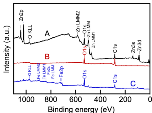
Fig. 10 XPS spectra of the original galvanized steel electrode (A), the same electrode utilized in the \text{CO}_2 electrolysis at 550\text{ }^\circ\text{C} in molten Li, K borate/Li, Na carbonate (1 : 1 mol/mol) blend (B), and the same electrode after cleaning its surface of the CNT deposited during the electrolysis (C). For electrolysis conditions, see Experimental.
