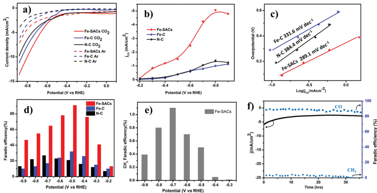
Fig. 2 \text{CO}_2\text{RR} catalytic performance of the as-synthesized catalysts. (a) LSV scans ( 5 \text{ mV s}^{-1} ) for the Fe-SACs, Fe-C, and N-C catalysts in Ar- and \text{CO}_2 -saturated \text{KHCO}_3 solutions (0.1 M). (b) Partial current density of Fe-SACs. (c) Tafel plots of the partial CO current density for relevant catalysts at different applied potentials. (d) Faradaic efficiencies (FEs) of CO and \text{H}_2 at various applied potentials on different catalysts. (e) FEs of \text{CH}_4 at different applied potentials for Fe-SACs and (f) long-term stability of Fe-SACs at a potential load of -0.5 \text{ V} vs. RHE and the corresponding FEs of CO and \text{CH}_4 .
