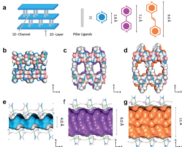
Fig. 7 (a) The crystal structure of [Cu_2(pzdc)L] . The pore constructed by three ligands of (b) and (e) CPL-1, (c) and (f) CPL-2, (d) and (g) CPL-5. 67 Reproduced from ref. 67 with permission, copyright The American Chemical Society, 2019.
