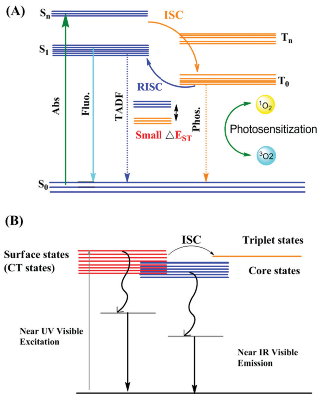
Fig. 1 Schematic illustration of Jablonski diagram (A) representing photophysical properties and ROS generation mechanism using organic dyes; adapted from ref. 18. (B) Proposed mechanism for the origin of luminescence in metal nanoclusters; adapted from ref. 11.
