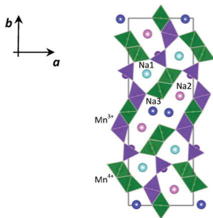
Fig. 1 The crystal structure of Na 0.44 MnO 2 , showing the ordering of Mn 3+ (violet) and Mn 4+ (green) ions and the presence of three distinct crystallographic sites for Na (Na1 cyan, Na2 pink, and Na3 blue).
