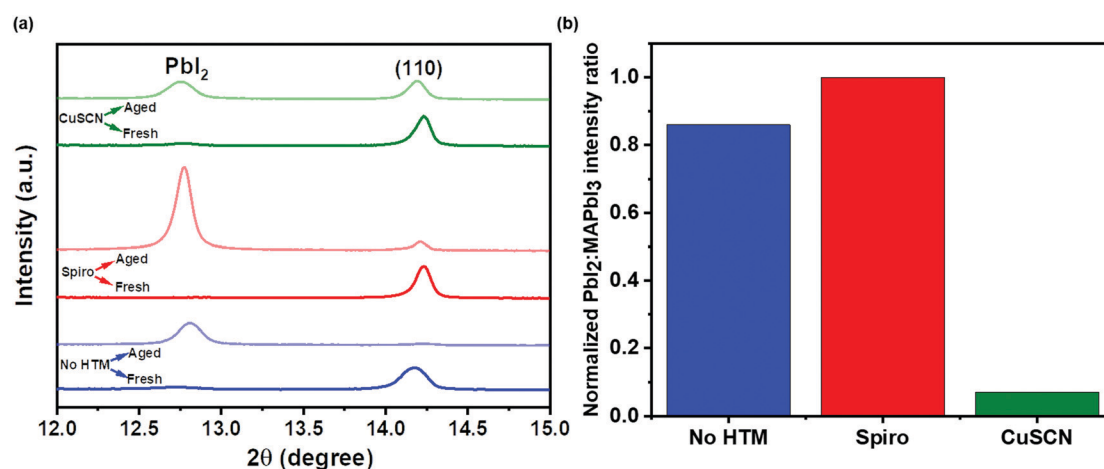
Fig. 4 (a) XRD pattern highlighting the Pbl 2 and (110) peak of MAPbI 3 fresh and aged PSC-HTM-free, PSC-spiro and PSC-CuSCN devices. (b) Normalized Pbl 2 :MAPbI 3 peak intensity ratios of the aged devices.
