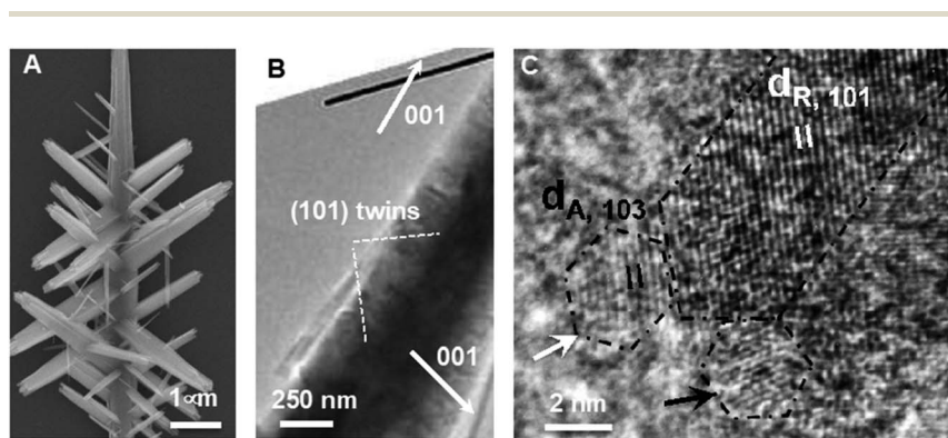
Fig. 6 Ex situ TEM data showing (A) a branched rutile nanowire, (B) the crystallographic relationship between the branches and trunk, and (C) attachment of the (103) faces of anatase nanoparticles onto the (101) faces of rutile nanowires, followed by transformation to rutile. 48 Reprinted with permission from ref. 48. Copyright 2013 American Chemical Society.
