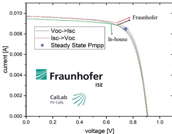
Fig. 3 \text{Cu}(\text{In,Ga})\text{S}_2/\text{(Zn,Sn)O}/\text{Al:ZnMgO}/\text{Al:ZnO} certified I - V curves of the 14.0% efficiency device measured at the Fraunhofer Institute for Solar Energy Systems. The red curve is the measurement from the short-circuit current to the external open-circuit voltage, and the black curve is the measurement from the external open-circuit voltage to the short-circuit current. The olive curve is the in-house measurement. The blue square point shows the steady-state maximum power-point of the device achieved by keeping the device at V_{\text{mpp}} for 5 minutes.
