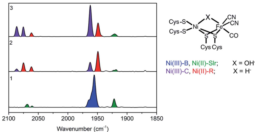
Fig. 2 (Left) Baseline corrected FTIR spectra of a DvMF [NiFe] hydrogenase as isolated 1 , incubated 4 hours in H_2 atmosphere 2 , and in 15 \mu\text{l} of viologen and 40 \mu\text{l} NaDT 3 . Band positions for the different state are as follows: Ni(III)-B ( 1955 , 2081 , and 2090 \text{ cm}^{-1} ), Ni(II)-Sl r ( 1922 , 2061 , 2070 \text{ cm}^{-1} ), Ni(III)-C ( 1961 , 2074 , 2085 \text{ cm}^{-1} ), Ni(II)-R ( 1948 , 2061 , 2074 \text{ cm}^{-1} ). (Right) Schematic representation of DvMF [NiFe] hydrogenase active site, where X is identified for each redox state.
