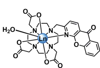
[\text{LnL}^{10}(\text{H}_2\text{O})]
