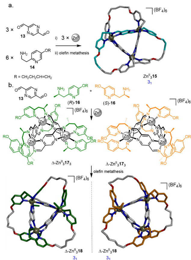
Fig. 6 (a) Synthesis of molecular trefoil knot Zn^{II}_{15} via a trimeric circular helicate. 53 (b) Chiral self-sorting of trefoil knots based on a pyrazine-2,5-dicarbaldehyde motif. 54
