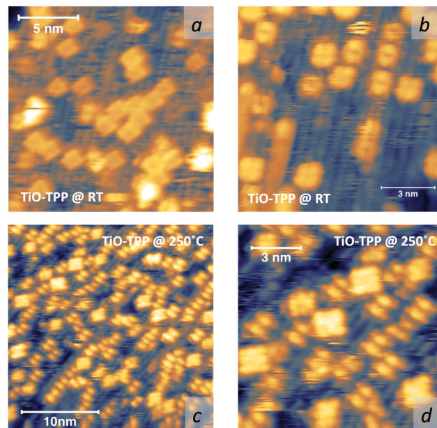
Fig. 21 Top: STM images (W tip) of a \sim 0.4 ML film of TiO-TPP deposited at RT: (a) the region is covered with a majority of square molecules adsorbed on the Ti_{5f} rows (bright rows) and rotated by 45°; a few saddle-shaped molecules with an overall dimmer intensity are observed on the O_{br} rows (+1.4 V, 150 pA); and (b) in this region, most of the molecules are adsorbed on the O_{br} rows with a saddle-shaped conformation, and a few molecules in between the O_{br} and Ti_{5f} rows rather display a four-leaf motif (+1.7 V, 190 pA). Bottom: The same film after annealing to 250 °C (+1.2 V, 170 pA): (c) most of the molecules are now observed on the O_{br} rows with a saddle-shape; and (d) close-up view of a few residual square-R45° molecules on Ti_{5f} rows, surrounded with saddle-shaped molecules on the O_{br} rows.
