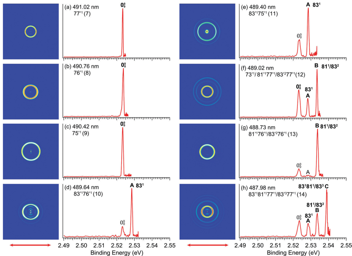
Fig. 6 Resonant photoelectron images and spectra of R -TFAE ^- at (a) 491.02 nm (2.5250 eV); (b) 490.76 nm (2.5264 eV); (c) 490.42 nm (2.5281 eV); (d) 489.64 nm (2.5322 eV); (e) 489.40 nm (2.5334 eV); (f) 489.02 nm (2.5354 eV); (g) 488.73 nm (2.5369 eV); (h) 487.98 nm (2.5408 eV). The vibrational Feshbach resonances (in parenthesis) and the assignments are given. The autodetachment-enhanced vibrational peaks are labelled in bold face.
