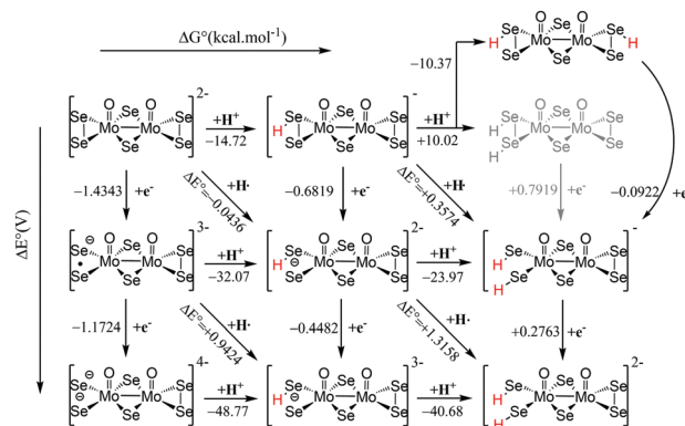
Fig. 3 Thermodynamic routes for compound [\text{Mo}_2\text{O}_2(\mu\text{-Se})_2(\text{Se}_2)_2]^{2-} 1 with two variables: electron addition (vertical) and proton addition (horizontal).
