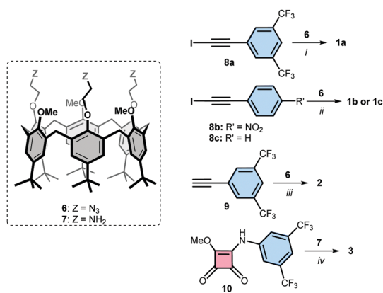
Scheme 1 Synthesis of receptors 1–3 from precursor calix[6]arenes 6 and 7 . Conditions: (i) CuI, TBTA, THF; (ii) [\text{Cu}(\text{CH}_3\text{CN})_6]\text{PF}_6 , TBTA, THF; (iii) [\text{Cu}(\text{CH}_3\text{CN})_6]\text{PF}_6 , 2,6-lutidine, DCM; (iv) DIPEA, MeOH, DCM.
