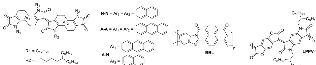
Fig. 23 Chemical structures of selected n-type thermoelectric fully fused polymer derivatives, including published synonyms.
