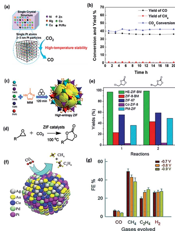
Fig. 15 (a) Schematic of the Pt/Ru- (\text{NiMgCuZnCo})\text{O} entropy-stabilized metal oxide solid solution synthesized by mechanical ball milling; (b) \text{CO}_2 hydrogenation stability of 5 wt% Pt doped HEO at 500^\circ\text{C} for 20 h. Reproduced with permission (ref. 175). Copyright 2019, American Chemical Society. Schematic of (c) ZIF HEM synthesized by the mechanochemistry method; (d) catalytic cycloaddition of \text{CO}_2 with epoxides to produce cyclic carbonates; and (e) yields of two cyclic carbonates obtained from the cycloaddition of \text{CO}_2 with corresponding epoxides catalysed by HE-ZIF-BM, ZIF-8-BM, ZIF-67, Cd-ZIF-8, and PM-ZIF. Reproduced with permission (ref. 190). Copyright 2019, Wiley-VCH. (f) Schematic of \text{CO}_2 conversion to hydrocarbon fuels on the Cu-based HEA catalyst; (g) bar diagram for the faradaic efficiencies of carbonaceous species and hydrogen gaseous products of the reaction. Reproduced with permission (ref. 191). Copyright 2020, American Chemical Society.
