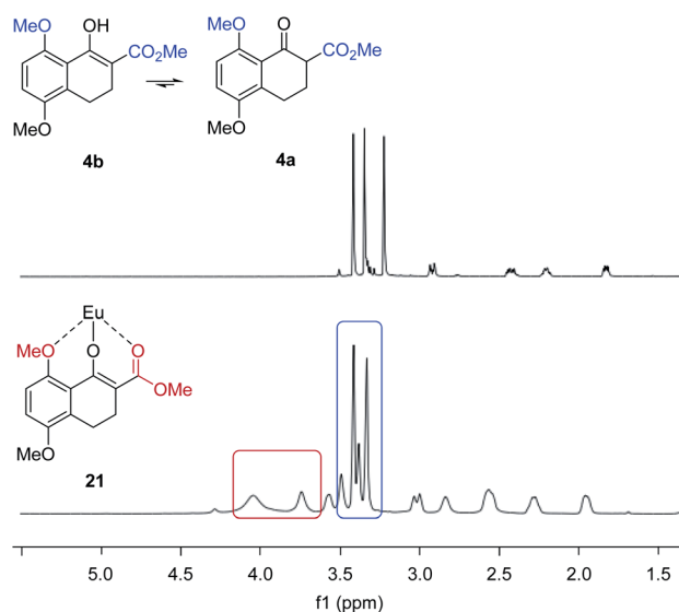
Fig. 6 \text{Eu}(\text{fod})_3 NMR shift reagent induces chemical shifts of the methyl groups in \beta -ketoester substrate 4.
