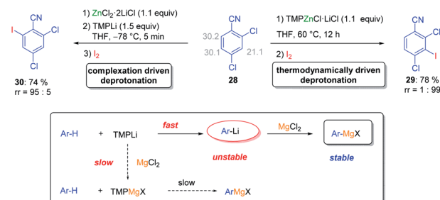
Scheme 15 Kinetic and thermodynamic deprotonation of aryl nitrile 28 .
