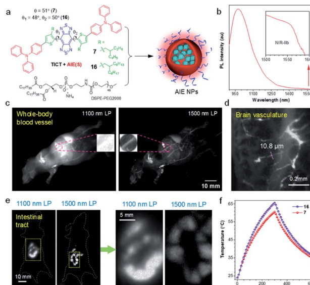
Fig. 5 (a) Schematic illustration for the preparation of AIE NPs from AIEgen 7 and 16 . (b) PL spectrum of AIE8 NPs. Inset: zoom-in emission spectra in the range of 1500–1600 nm. (c) Comparison of NIR-II fluorescence signal for whole-body imaging of living mice in an area close to liver under 1100 and 1500 nm LP filters, respectively (AIE7 NPs, 200 \mu\text{L} , 0.8 \text{mg mL}^{-1} ). Inset: zoom-in images of the blood vessel. (d) High-magnification through-skull microscopic imaging of the brain vasculature. (e) NIR-II fluorescence images of the intestinal tract using 1100 and 1500 nm LP filters, respectively (AIE7 NPs, 300 \mu\text{L} , 1 \text{mg mL}^{-1} ). Right: zoom-in images of the two yellow rectangle areas. (f) Comparison of the photothermal properties of 7 and 16 NPs. Data adapted with permission. 66 Copyright, 2020, Nature Publishing Group.
